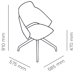
ICON HIGH BACK SWIVEL swivel, 4-spoke base girevole, base a 4 razze 7150
